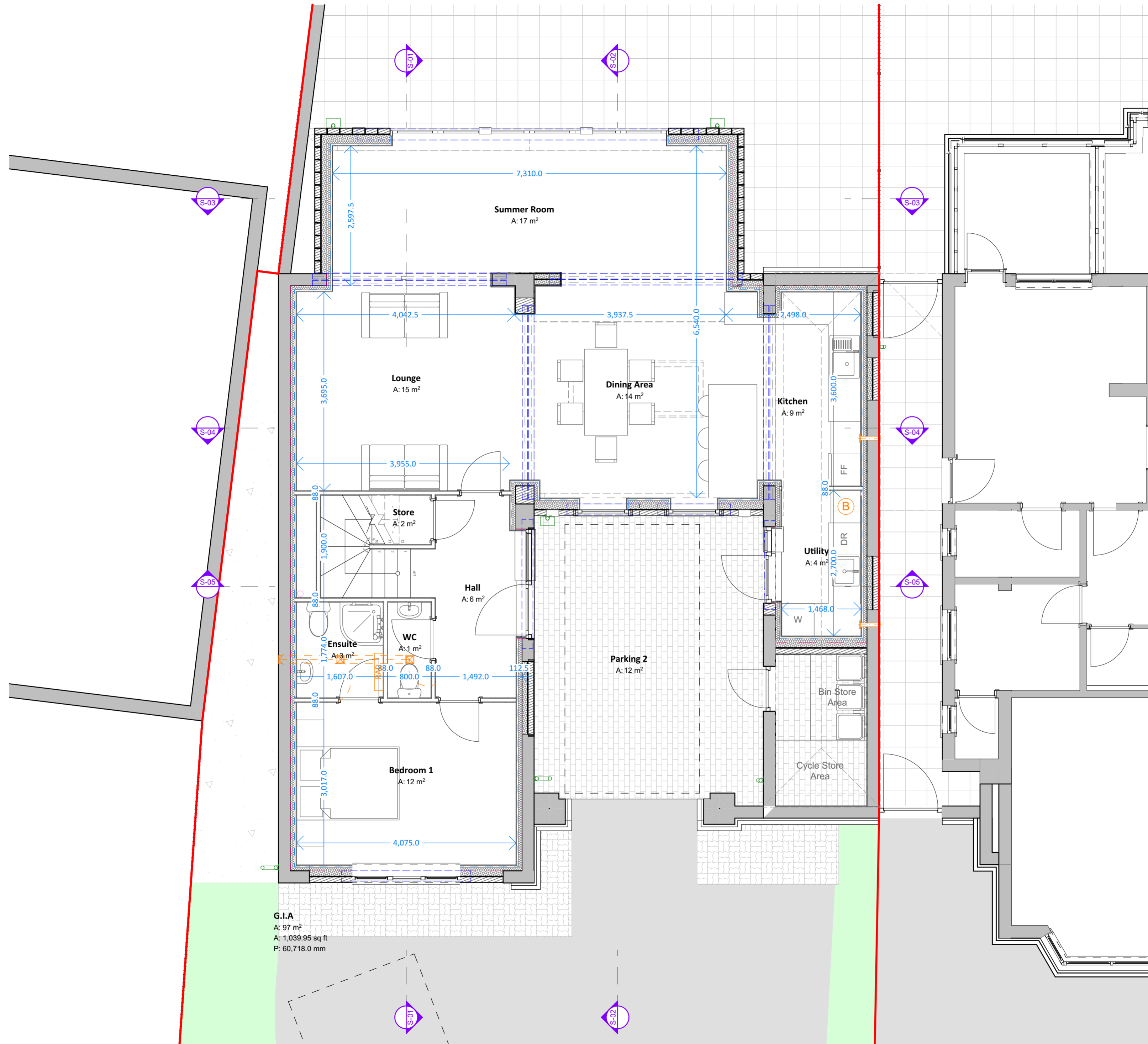
0. Ground Floor 1:50
