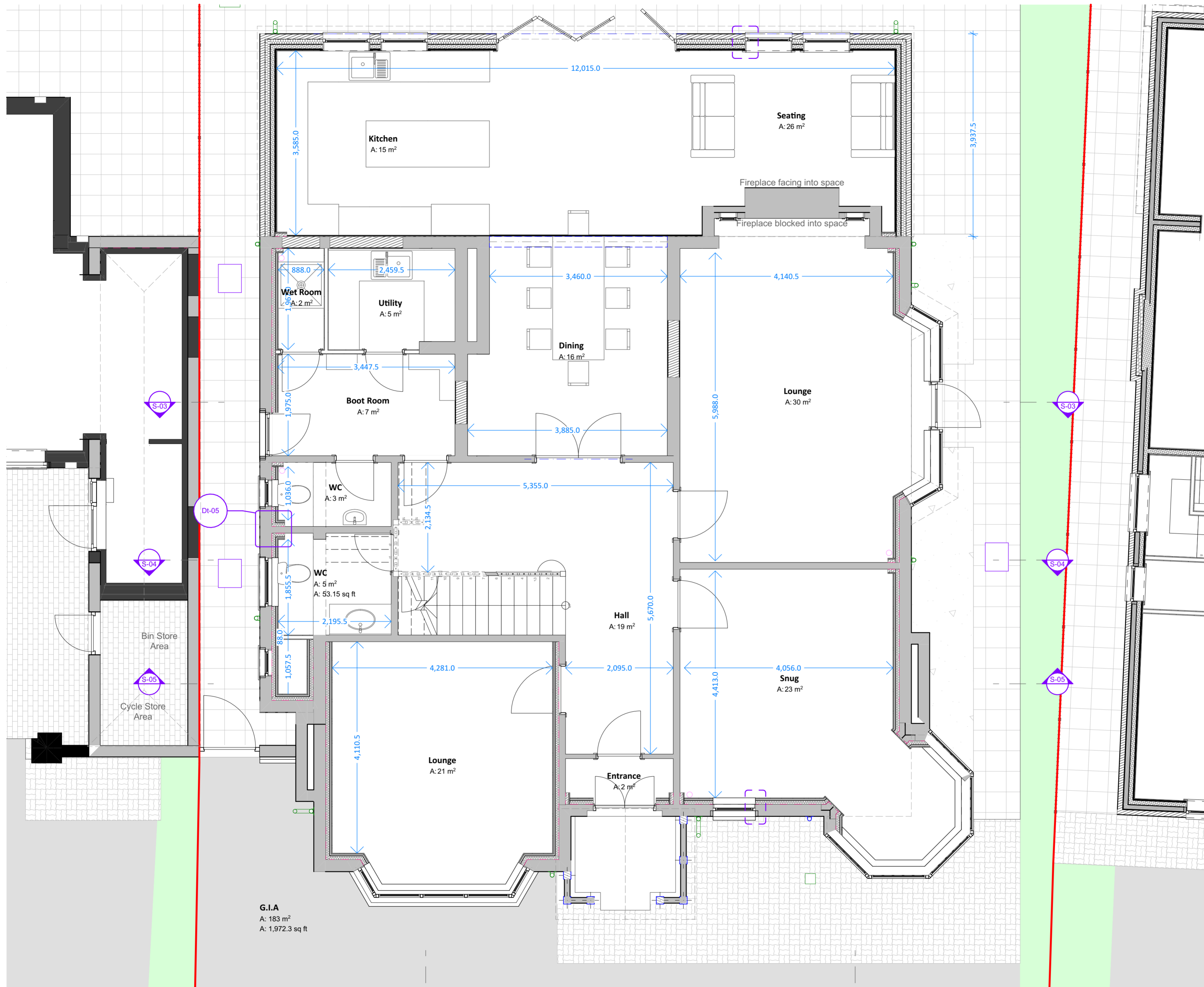
0. Ground Floor 1:50
