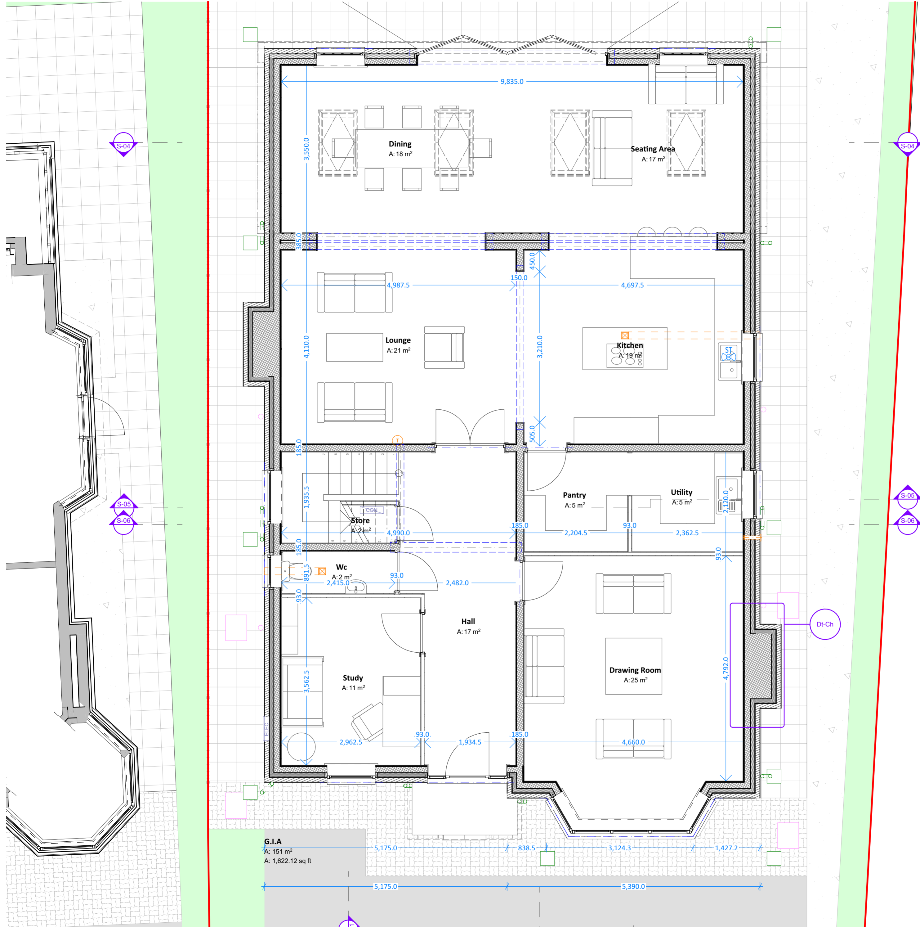
0. Ground Floor 1:50
